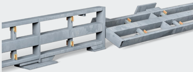
Tipping length limitation (KLB element)
