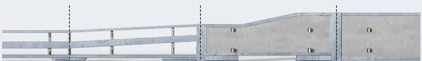
Transition element ProTec 50 to ProTec 120/121
